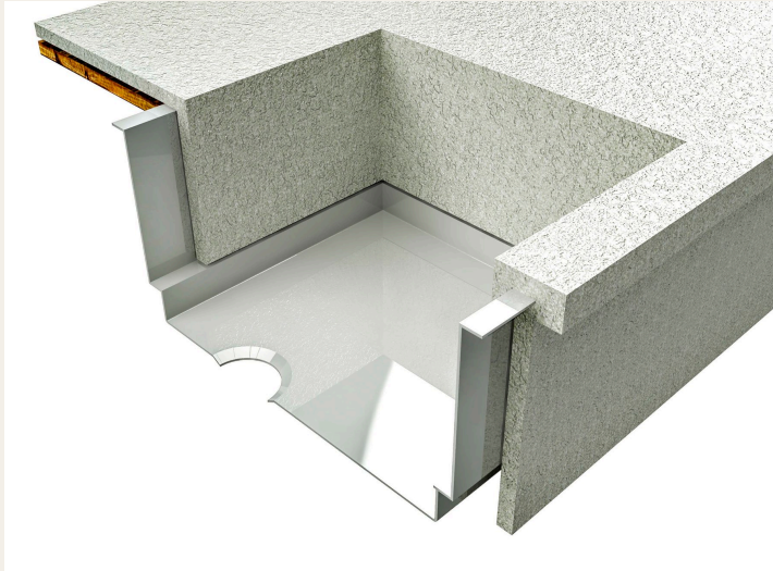
Cutaway: stone deck and walls over the stainless Capstone body.
